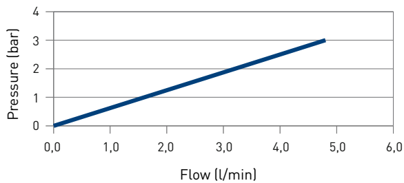
Flow - Pressure characteristics
